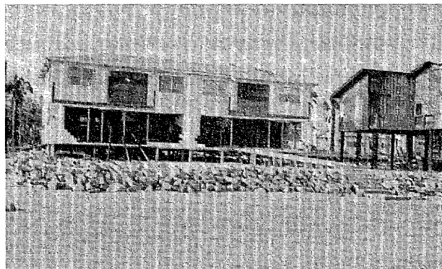
Exceeding minimum building requirements, this home performed well compared to its neighbors during Hurricane Hugo (1989).
