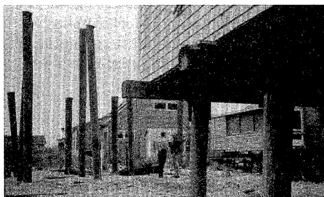
Piles are generally made of wood or prestressed concrete. They often are braced against lateral and shear forces using wood knee and cross bracing, steel rods, and guy wires.
