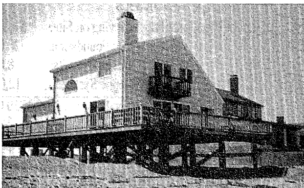
Flexible connections between building support beams and wooden piles allow adjustments to be made to account for imperfect pile driving.
