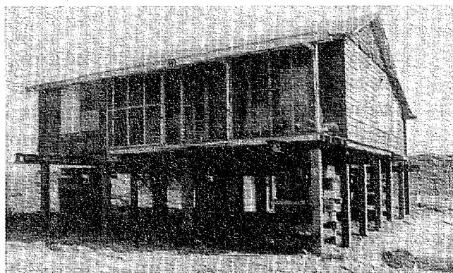
A home to be relocated is supported on cribbing prior to lowering onto a wood post foundation.
