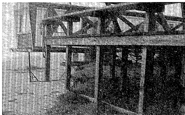
The Corps of Engineers estimates that Washaway Beach, Washington, is experiencing the fastest rate of coastal erosion in the U.S.
