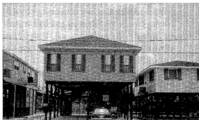
The home is set on the new pile foundation system.
